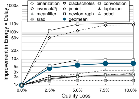
Figure 12: Energy-delay benefits vs output quality (log scale).
